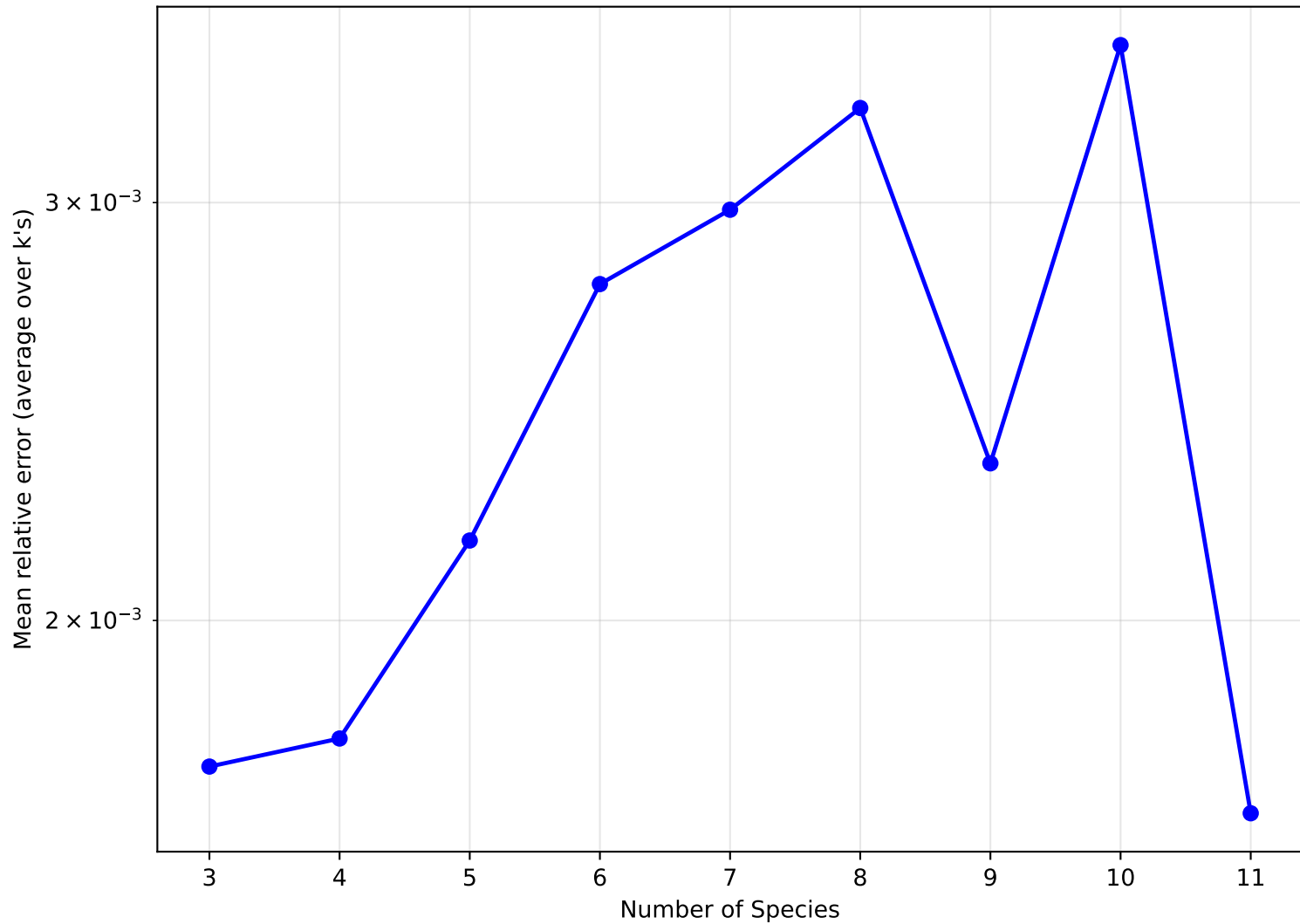
30, 30 — Mean relative error vs number of species
